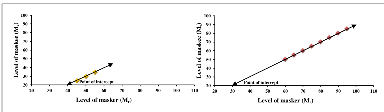
Fig. 2. Establishment of the point of interception from two extreme points. This point of intercept is considered as the threshold of octave masking. The graph left indicates the intercept point of the level of masker with respect to the initial shift in the level of maskee. The graph right shows the intercept point of the level of masker with respect to the level of maskee taken after a gap of 15 dB visualized.
