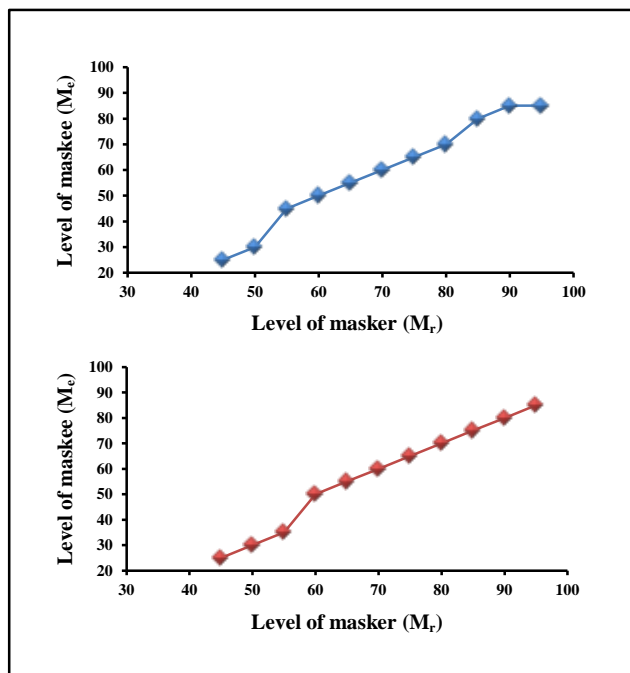
Fig. 1. Level of masker vs. level of maskee graph of a random subject (left ear: above and right ear: below) plotted to extract the intercept point and establish the threshold of octave masking.
